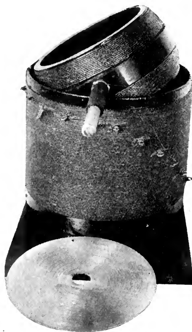
A SUITABLE VARIOCOUPLER For broadcasting or amateur reception, with its metal shield which reduces body capacity effects
